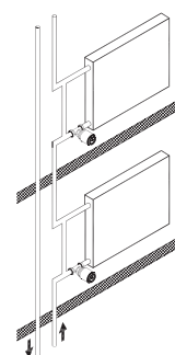
2. One-pipe system, flow from bottom
